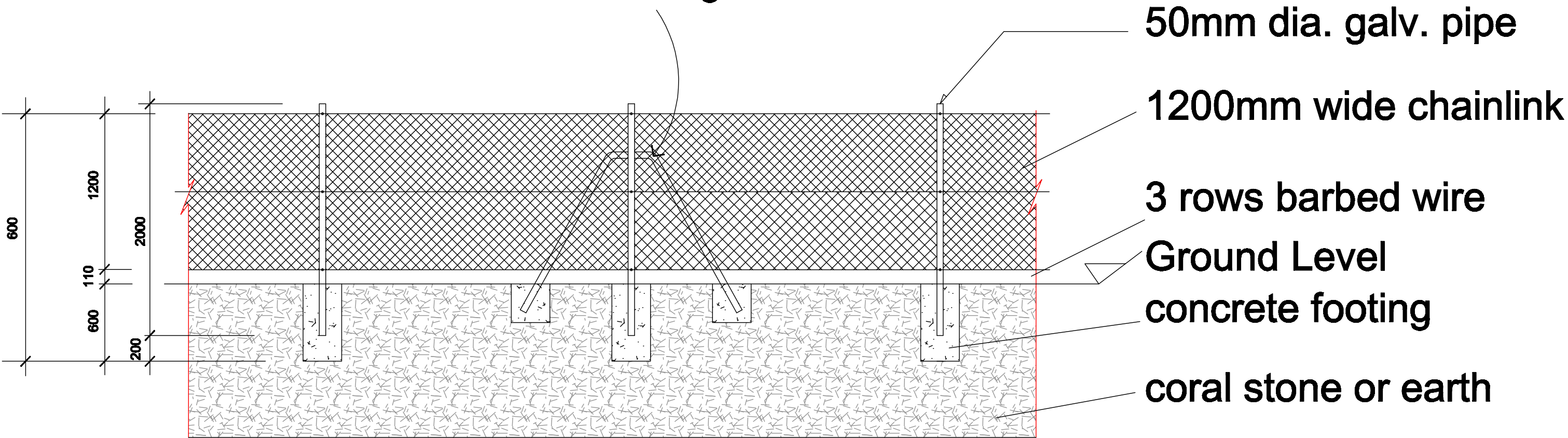
TYPICAL SECTIONAL ELEVATION
